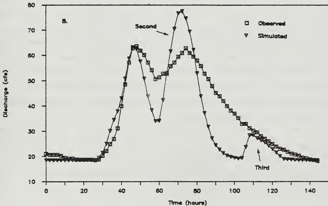
Figure 7. (A) Hietograph, and (B) simulated and observed hydrographs for a "complex" rainfall event on Deer Creek, Oregon Coast Range. The SCS method over-emphasizes the effects of a second and a third "pulse" of precipitation.
